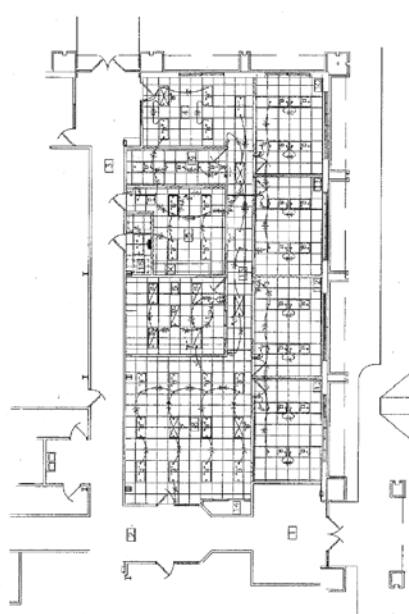
LIGHTING/FIRE ALARM PLAN SCALE: 1/8" = 1'-0"
